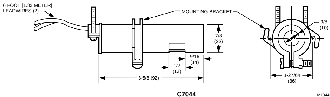
Fig. 3. Installation dimensions of C7044A in in. (mm).
