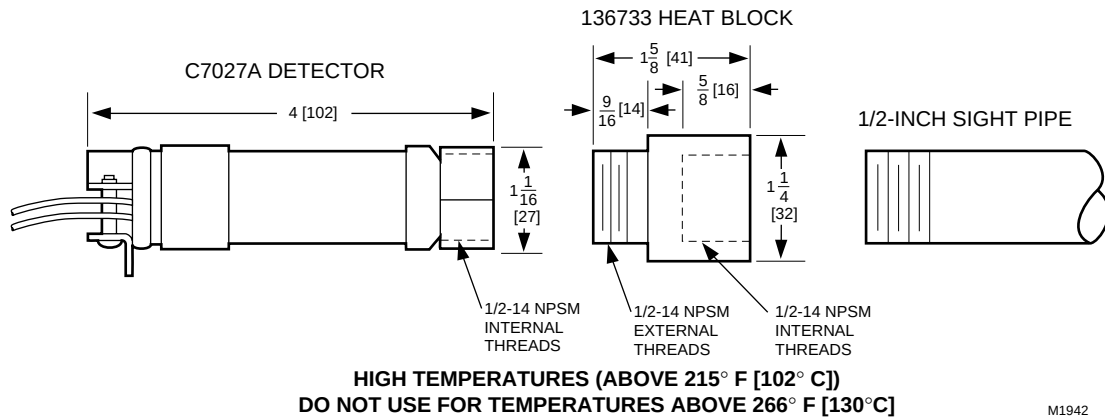
Fig. 7. Mounting dimensions of 136733 Heat Block in. (mm).
