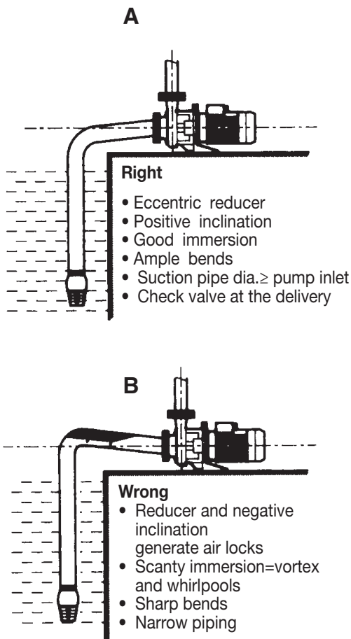
fig. 1 - Pump installation
