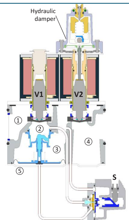
Sectional drawing of multifunctional gas valve M2C**S
