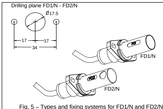
Fig. 5 – Types and fixing systems for FD1/N and FD2/N
