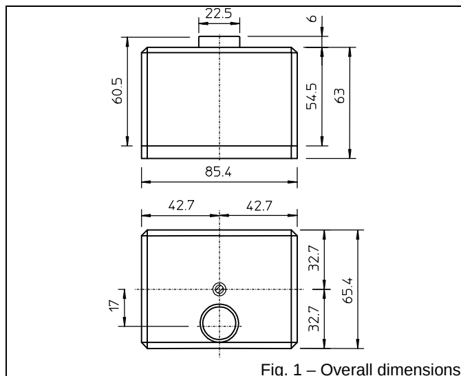
Fig. 1 – Overall dimensions
