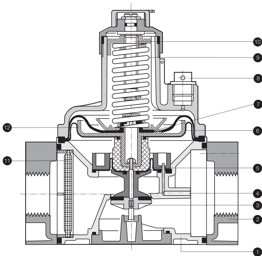
FRI sectional drawing Shown in closed position
