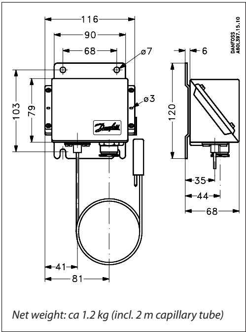
KPS with remote sensor
