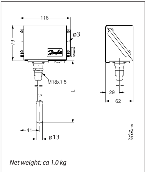
KPS with rigid sensor
