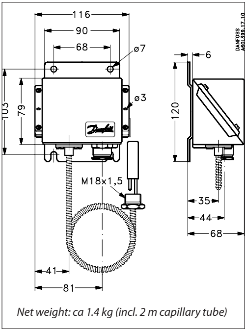
KPS with remote sensor and armoured capillary tube
