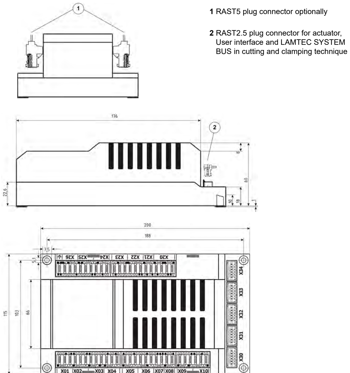
Fig. 2 Dimensions BT320 ... 341 (terminal assignment BT330/BT341 only)
