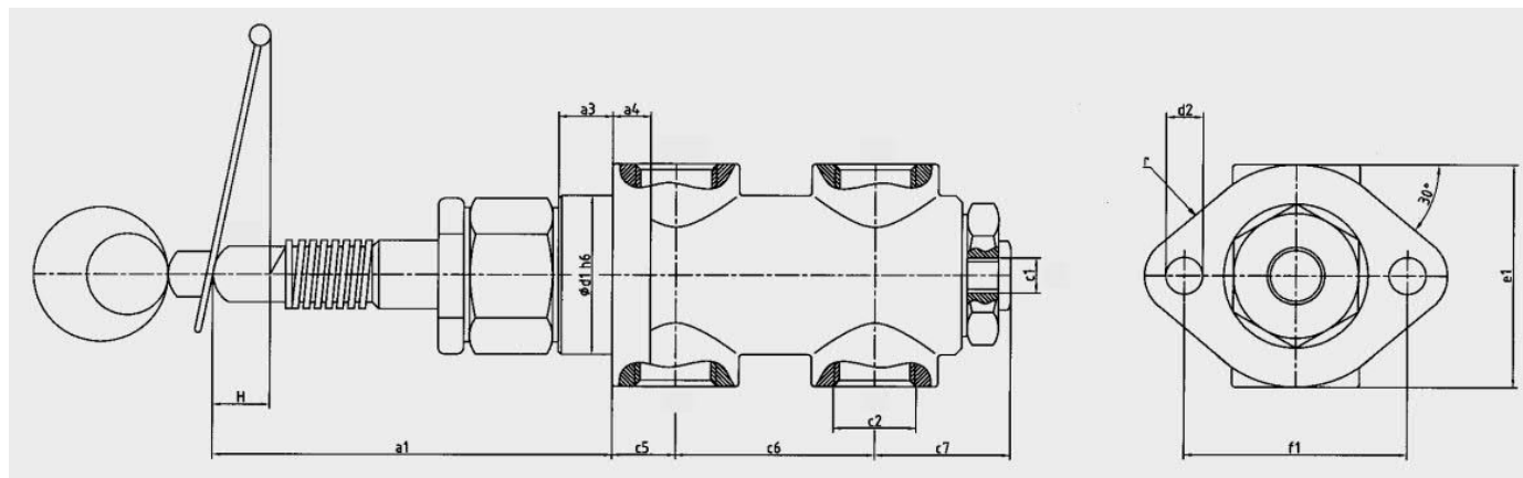
Fig.2 Dimensions
